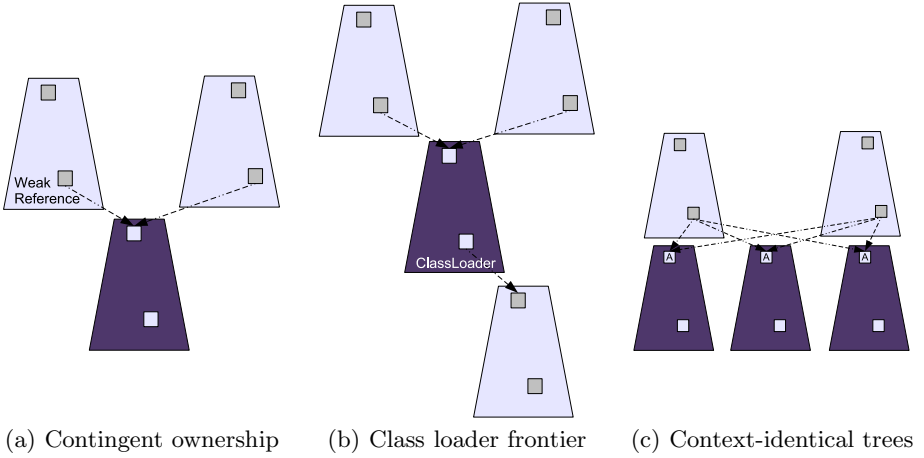
Fig. 3. Three common semantic properties of graphs
