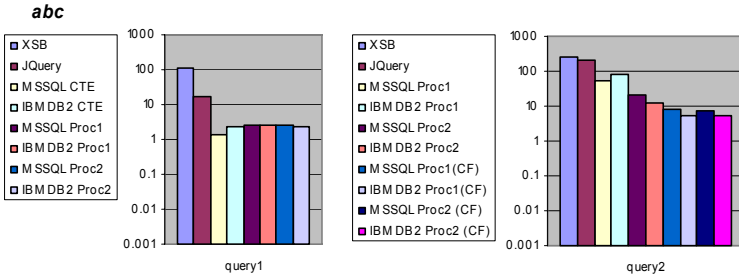
Fig. 2. Project specific queries evaluation times
