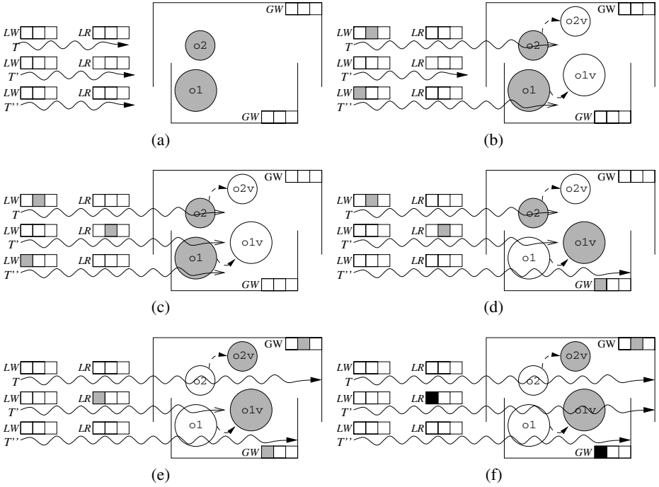
Fig. 4. A non-serializable execution
